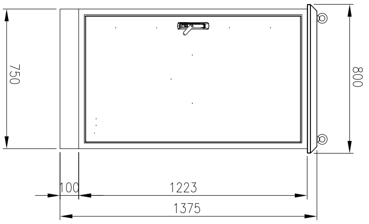
FRONT VIEW (ASSEMBLY)
