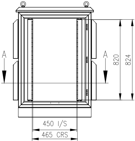
FRONT VIEW (FRONT DOOR REMOVED)
