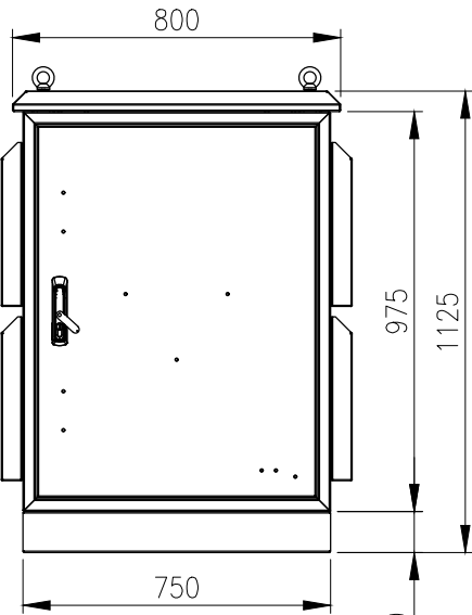
FRONT VIEW (ASSEMBLY)
