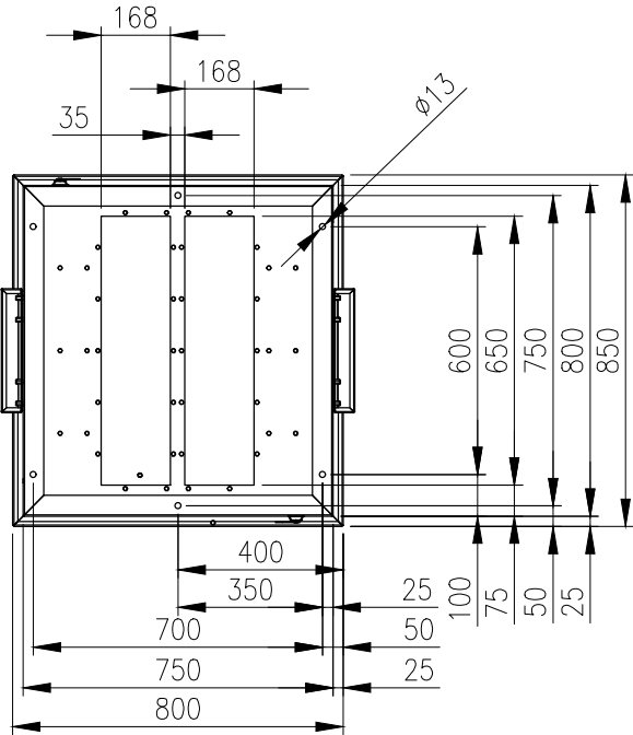
BOTTOM VIEW
