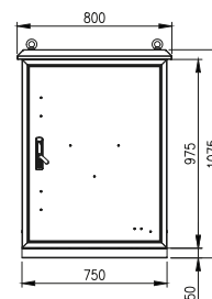
FRONT VIEW (ASSEMBLY)
