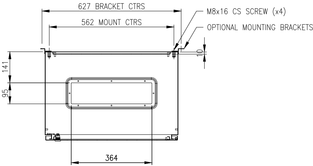
SECTION AW-AW
