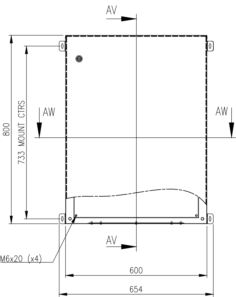
FRONT VIEW
