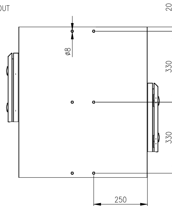
REAR VIEW
