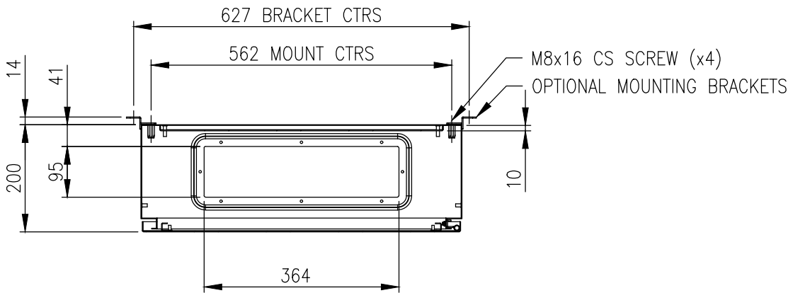
SECTION AW-AW
