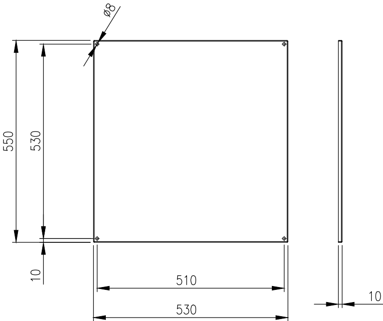
DEVICE MOUNTING PLATE
