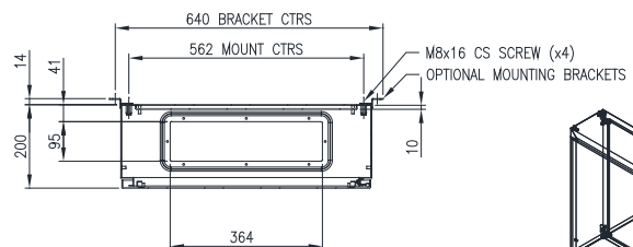
SECTION AW-AW
