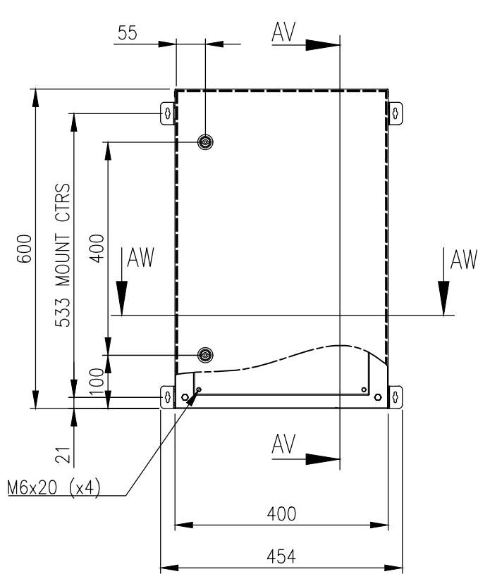
FRONT VIEW
