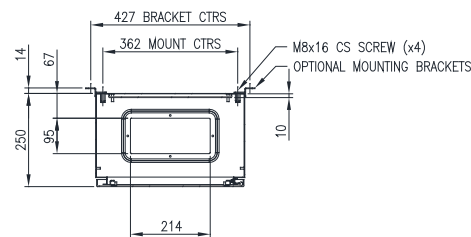
SECTION AW-AW
