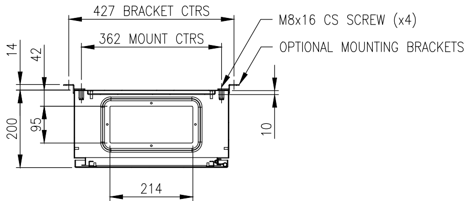
SECTION AW-AW
