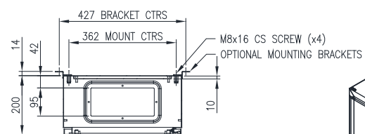
SECTION AW-AW
