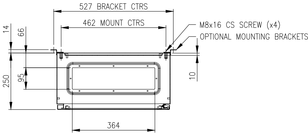
SECTION AW-AW
