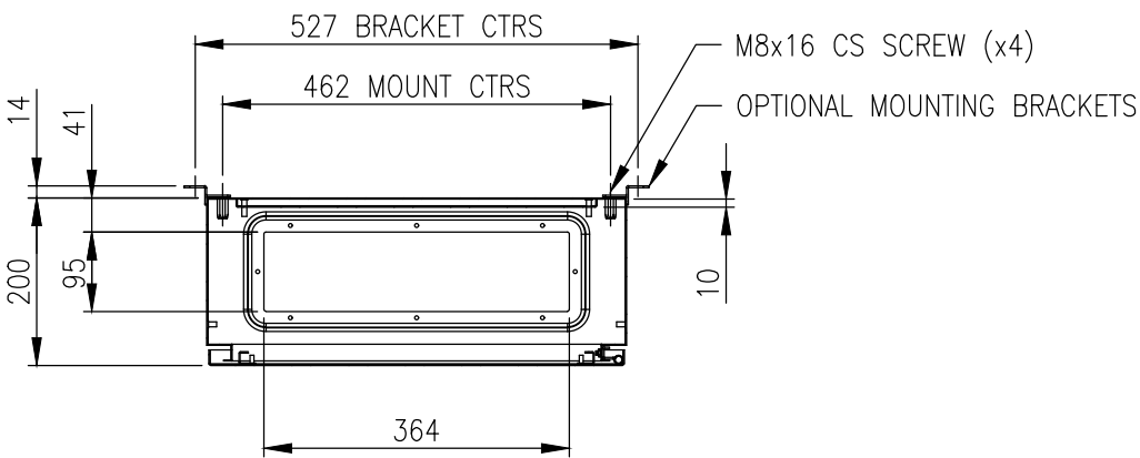
SECTION AW-AW
