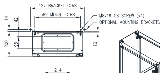
SECTION AW-AW
