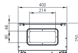
SECTION AW-AW
