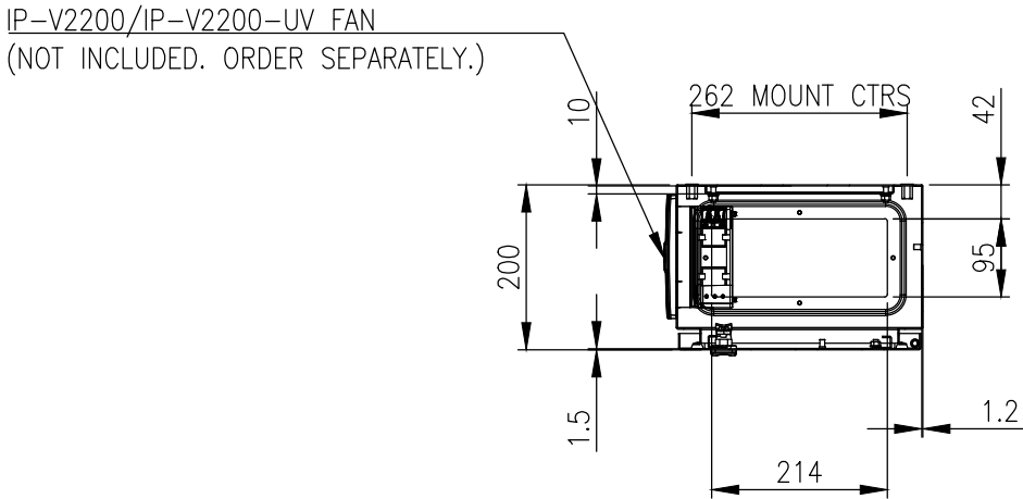
SECTION AW-AW
