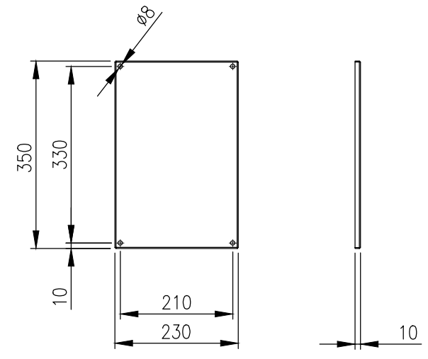
DEVICE MOUNTING PLATE
