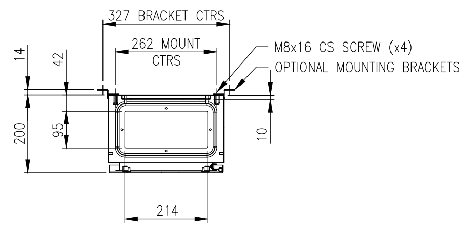
SECTION AW-AW
