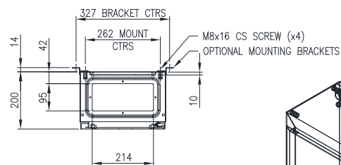
SECTION AW-AW
