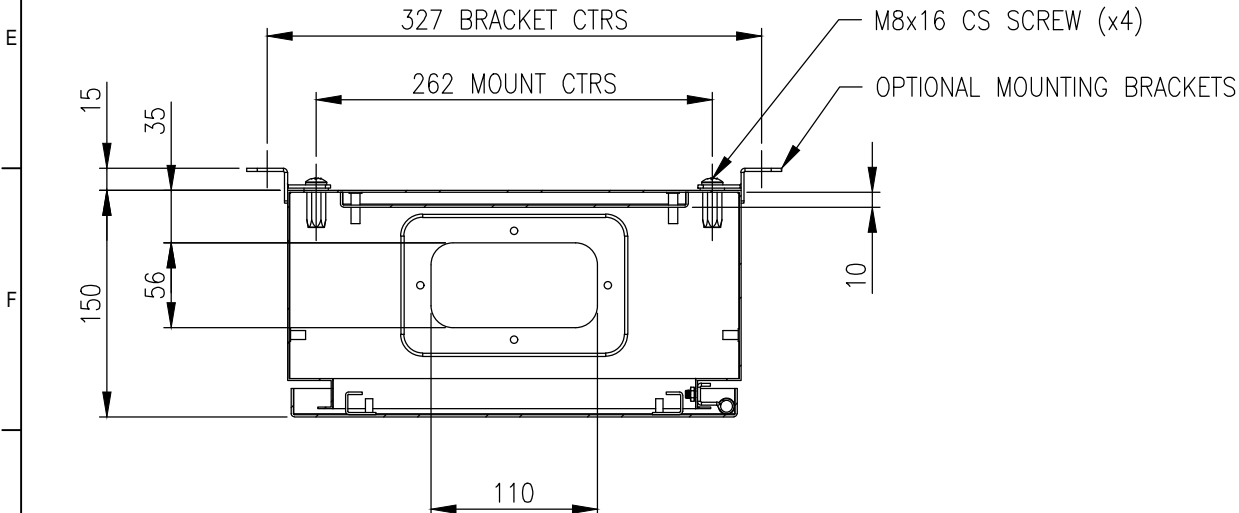
SECTION AW-AW
