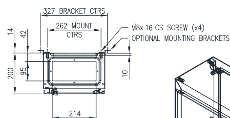
SECTION AW-AW
