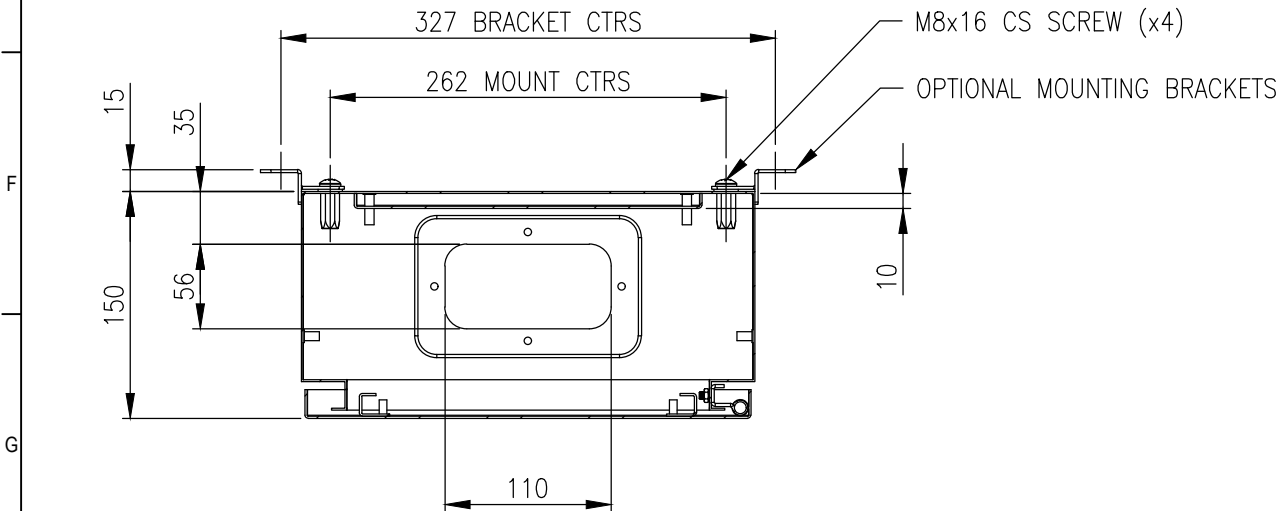
SECTION AW-AW
