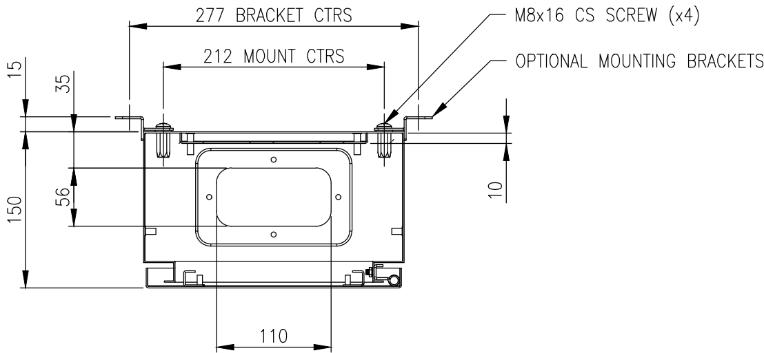
SECTION AW-AW
