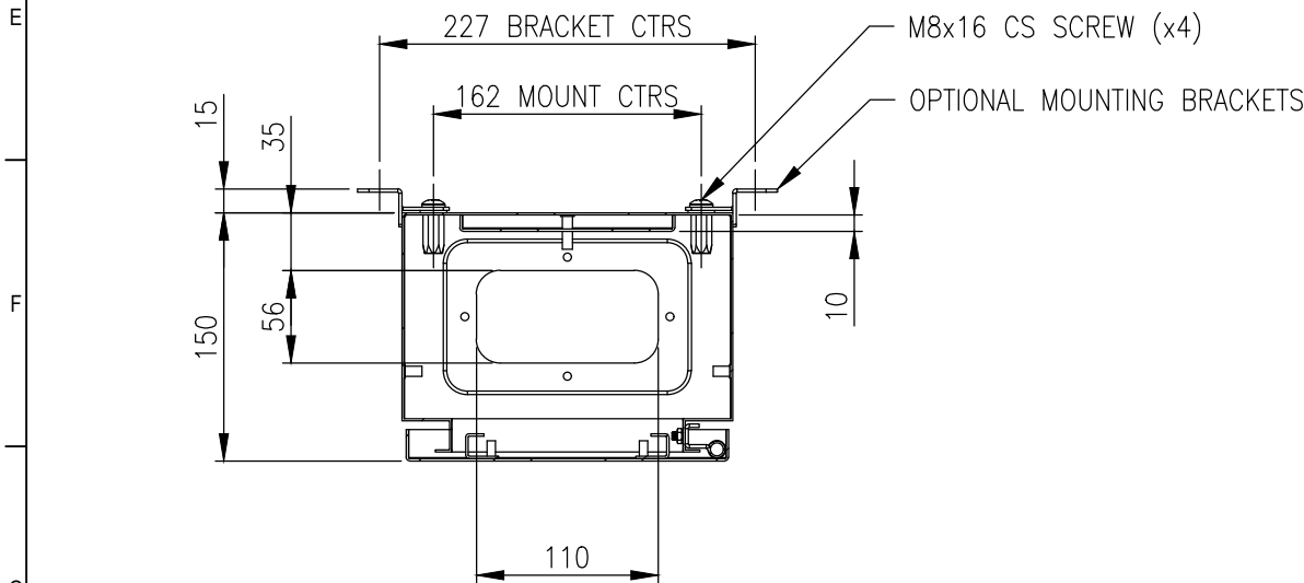
SECTION AW-AW
