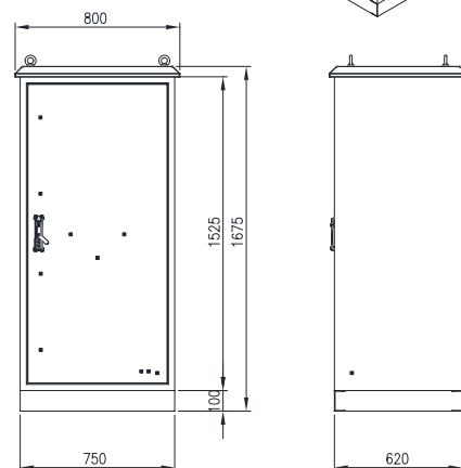
FRONT VIEW (ASSEMBLY)
