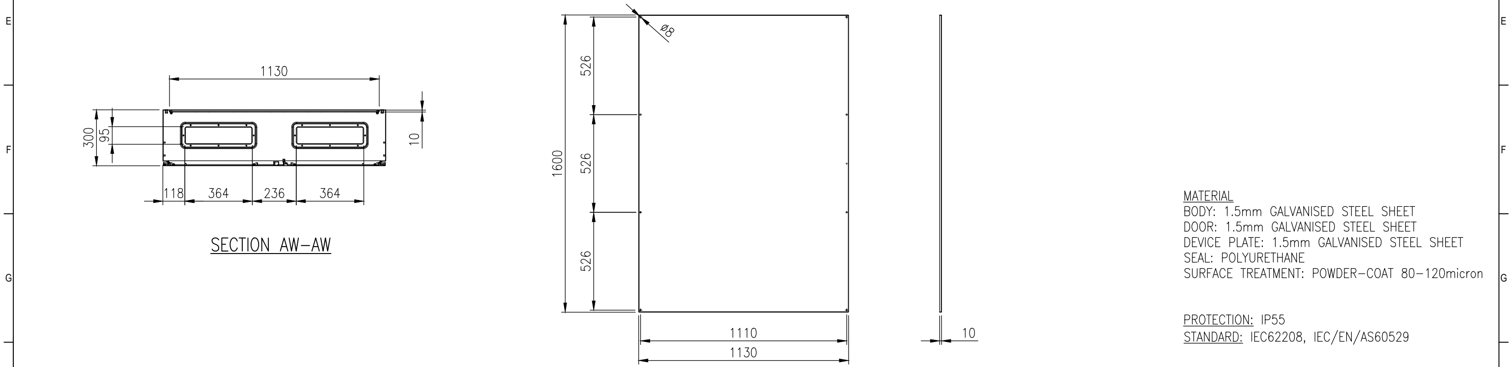
SECTION AW-AWDEVICE MOUNTING PLATE
