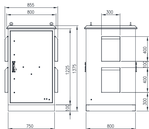
FRONT VIEW (ASSEMBLY)
