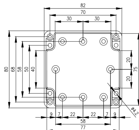
FRONT VIEW-DOOR REMOVED
